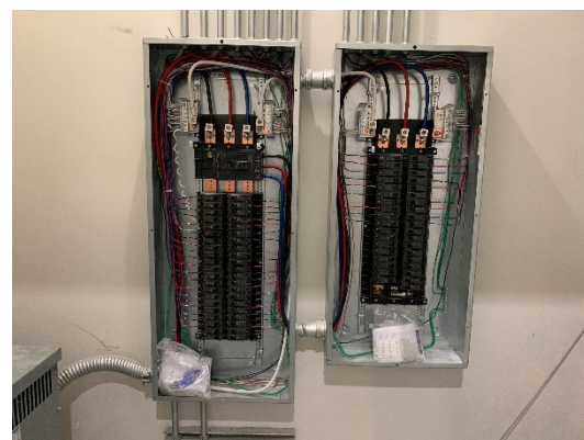
Breaker Box In New Addition
